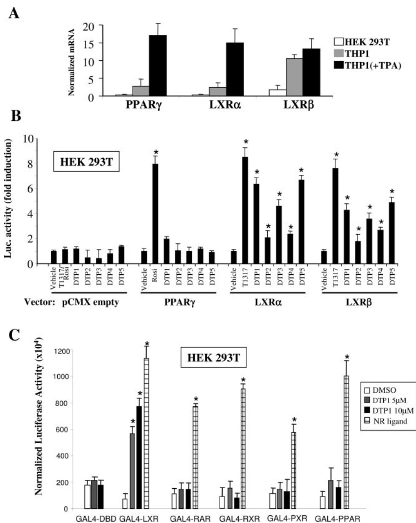
Fig. 1. Activation of LXR \alpha and LXR \beta by acanthoic acid-related DTPs. A , HEK 293T, THP-1, or THP-1 cells pretreated for 24 h with 20 nM TPA to promote differentiation into macrophages were maintained in culture, and the mRNA levels of PPAR \gamma , LXR \alpha , and LXR \beta were determined by quantitative RT-PCR. B , HEK 293T cells were cotransfected with the indicated pCMX nuclear receptor expression vectors, including RXR and the corresponding response element linked to a luciferase reporter gene. After transfection, cells were stimulated for 24 h with 1 \mu M rosiglitazone, 1 \mu M T1317, and 10 \mu M concentration of the indicated DTPs, and the luciferase activity was measured in the cell extracts. C , HEK 293T cells were transfected with a synthetic promoter containing four copies of the GAL4 response element and the GAL4 DBD fused to LXR \alpha , retinoic acid receptor \alpha , RXR \alpha , pregnane X receptor, or PPAR \gamma and stimulated for 24h with DTP1 (concentrations, 5 and 10 \mu M) and the corresponding nuclear receptor agonists (1 \mu M GW3965, 100 nM AM580, 50 nM LG268, 5 \mu M rifampicin, and 1 \mu M rosiglitazone). Results show the mean \pm S.D. of at least three experiments. *, P < 0.05 versus the condition with vehicle.
