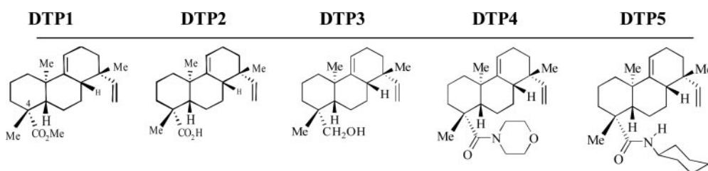
Fig. 2. Chemical structure and proposed generic names of acanthoic acid-derived DTPs modified at the C4 position used in this study. DTP1, diterpene methyl ester; DTP2, diterpene carboxylic acid; DTP3, diterpene methyl alcohol; DTP4, diterpene carboxyl morpholine; DTP5, diterpene carboxyl piperidine.
